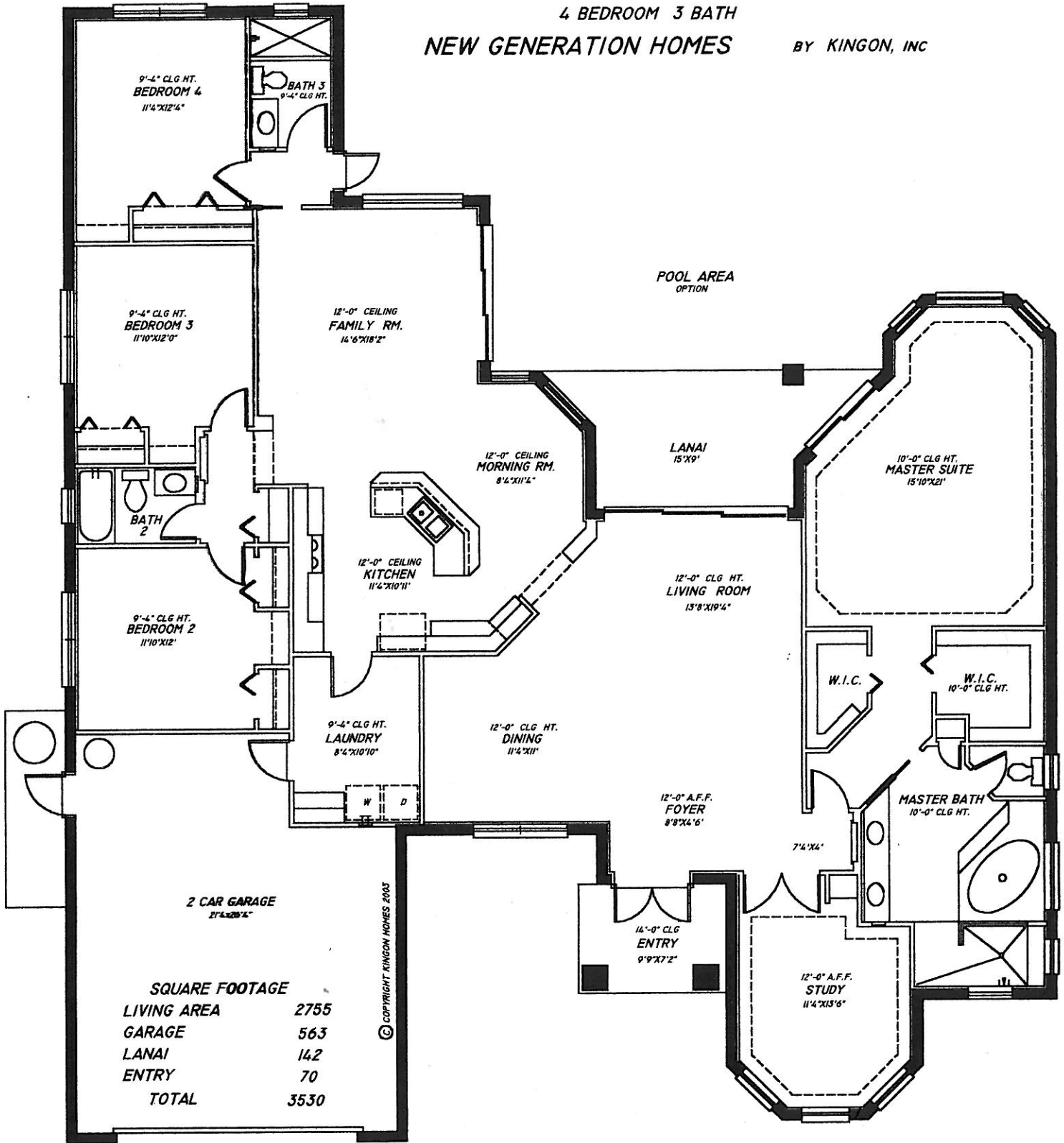
FLOOR PLAN
